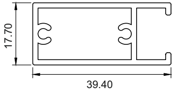
Shutter Vertical (Handle)
