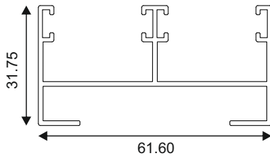
2 Track Top / Side
