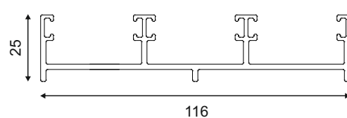
3 Track top
